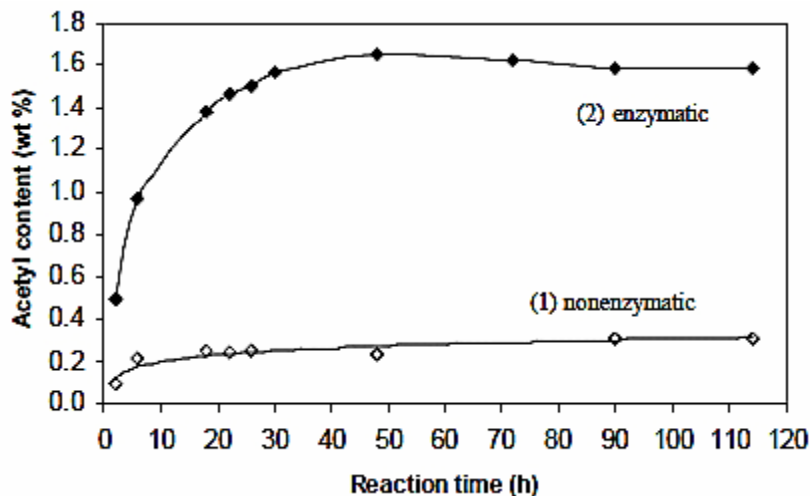
Figure 17. Time courses of CMC acetylation in aqueous medium with and without enzyme [78].
