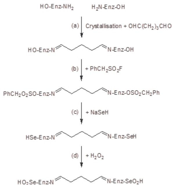
Figure 31. The preparation of CLCs of the semi-synthetic peroxidase seleno-subtilisin (a) batch crystallisation in 12% (w/v) \text{Na}_2\text{SO}_4 at 16-18°C was followed by treatment (45 min) with glutardialdehyde at pH 7.5; (b) 1h in 0.11M phenylmethanesulphonyl fluoride at pH 7.0; (c) addition of aqueous sodium hydrogen selenide solution was followed by 45h stirring at 45°C; and (d) 30 min in 10mM \text{H}_2\text{O}_2 . Enz, enzyme; Enz-OH, Ser221 of subtilisin; Enz-NH 2 , lysine residues on the surface of the enzyme; Ph, phenyl [107].
