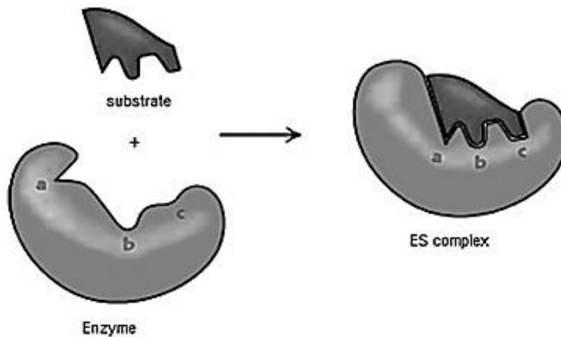
Figure 4. Induced-fit model of enzyme-substrate binding [30].
