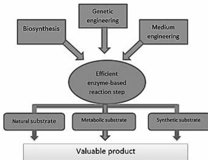
Figure 2. Rationale of the development of an enzymatic reaction step in organic synthesis [29].
