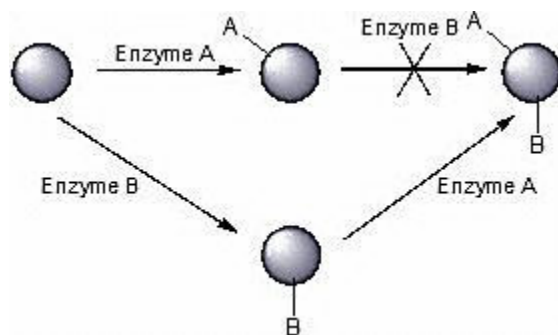
Figure 23. Orthogonality of biocatalysts [97].
