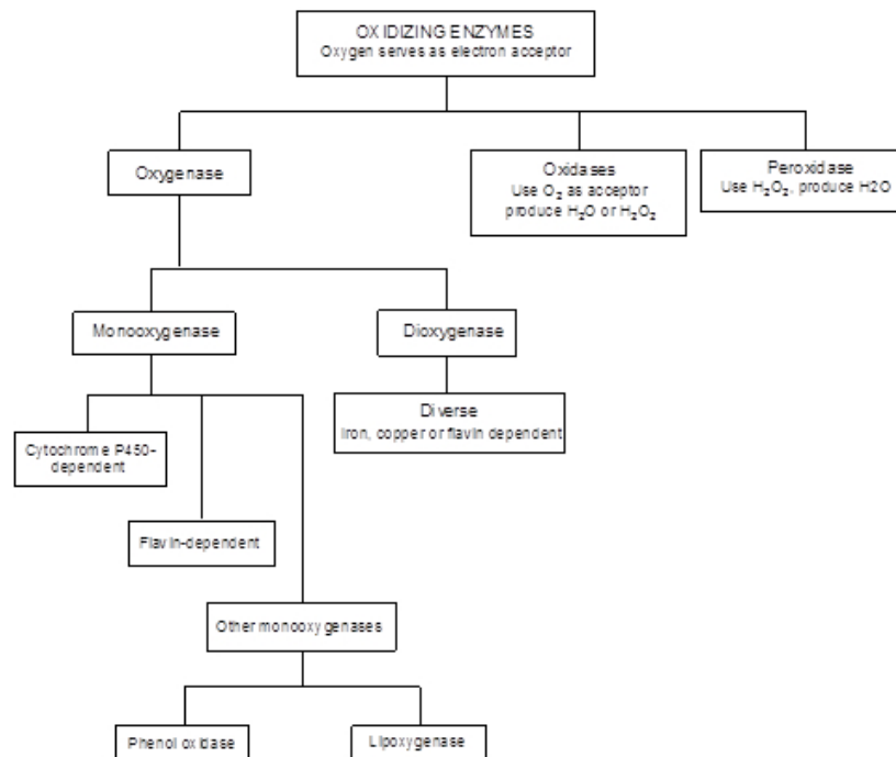
Figure 6. Classification of oxidizing enzymes [17].
