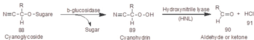
Figure 20. Role of hydroxynitrile lyase in cyanogenesis of higher plants [91].
