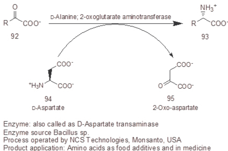
Figure 21. Enzymatic transformation catalyzed by a transferase [18].
