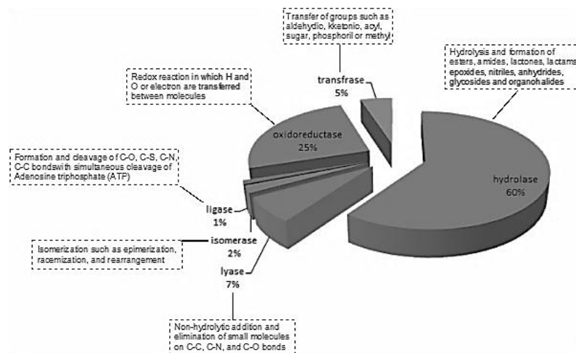
Figure 5. Classification of enzymes [31].
