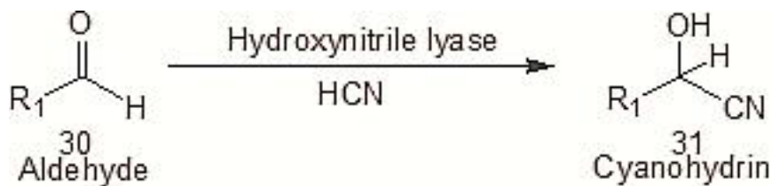
Figure 10. General reaction catalyzed by hydroxynitrile lyase [43].
