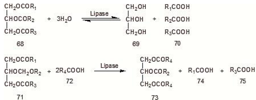
Figure 16. Examples of lipase-catalyzed reactions of triacylglycerols [2].
