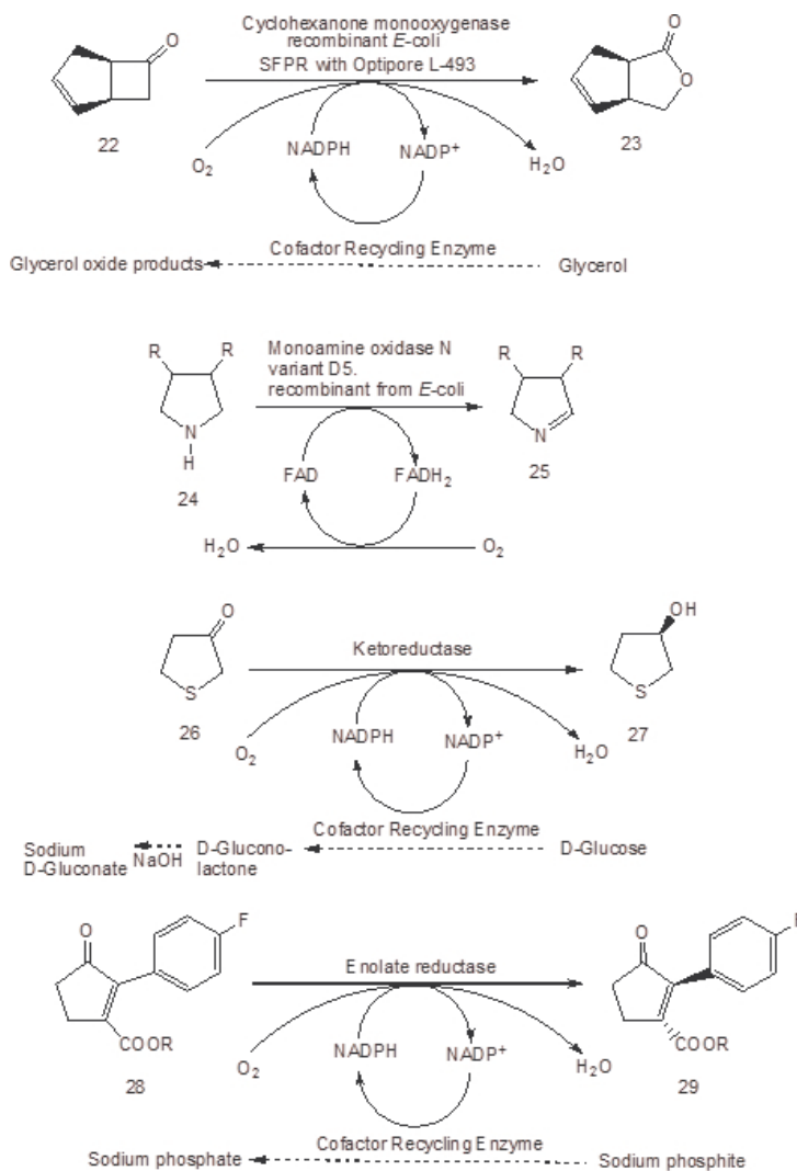
Figure 9. Selected biocatalytic oxidation and reduction reactions [42].
