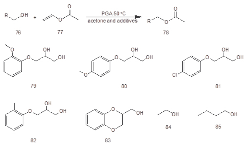
Figure 18. N-methylimidazole manipulates PGA to catalyze esterification [80].
