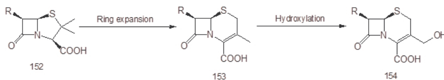
Figure 37. A non-heme iron (II) and 2-oxoglutarate-dependent cephalosporin C synthase in eukaryotes catalyzes two different catalytic steps with the same active site [124].
