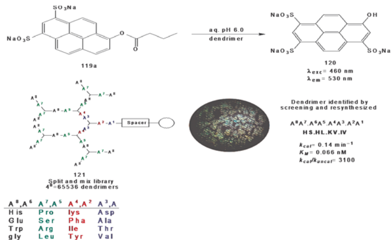
Figure 28. Combinatorial library of peptide dendrimers [28].
