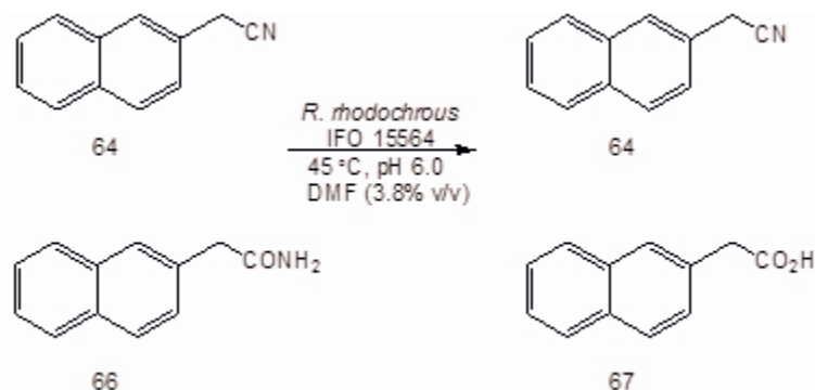
Figure 15. Preferential action of amidase of R. rhodochrous IFO 15564 on the mixture of a nitrile and an amide [47].
