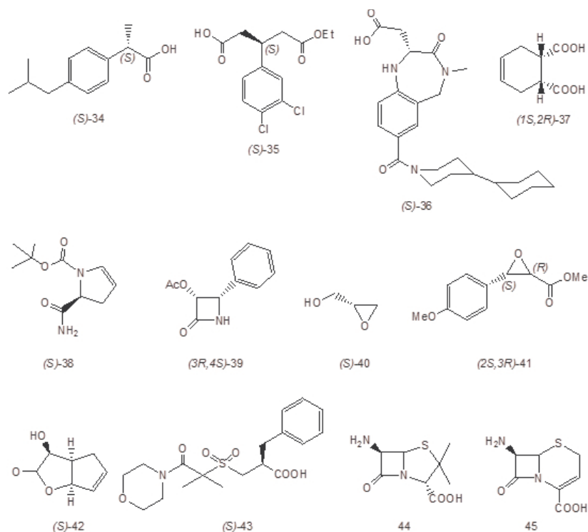
Figure 12. Some chiral building blocks obtained via hydrolase catalyzed-biotransformations [8].
