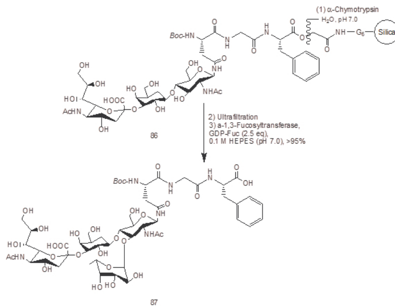
Figure 19. Chymotrypsin catalyzed release of glycopeptides from the solid support [87].
