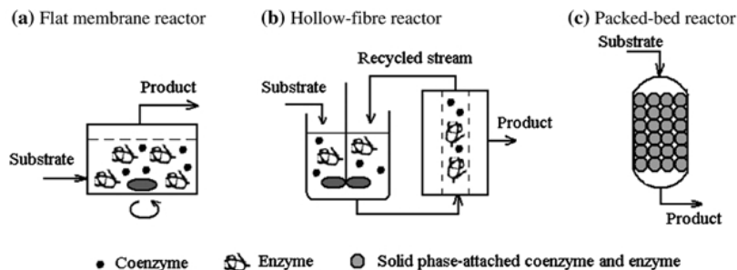
Figure 35. Typical configurations for sustainable cofactor retention in continuous-flow bioreactors [118].
