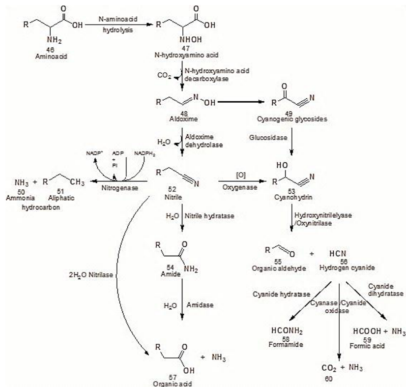
Figure 13. Metabolic pathways for nitrile synthesis and degradation in micro-organisms [48].
