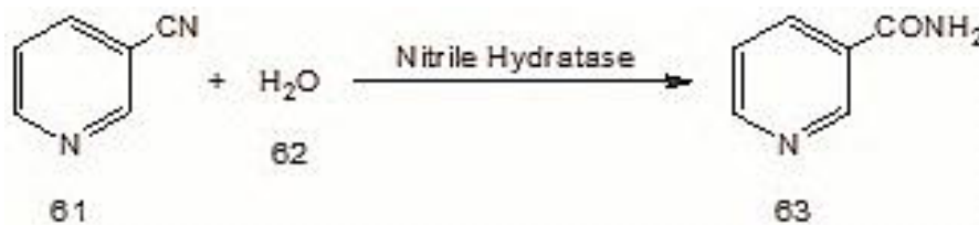
Figure 14. Enzymatic preparation of nicotinamide from 3-cyanopyridine [49].
