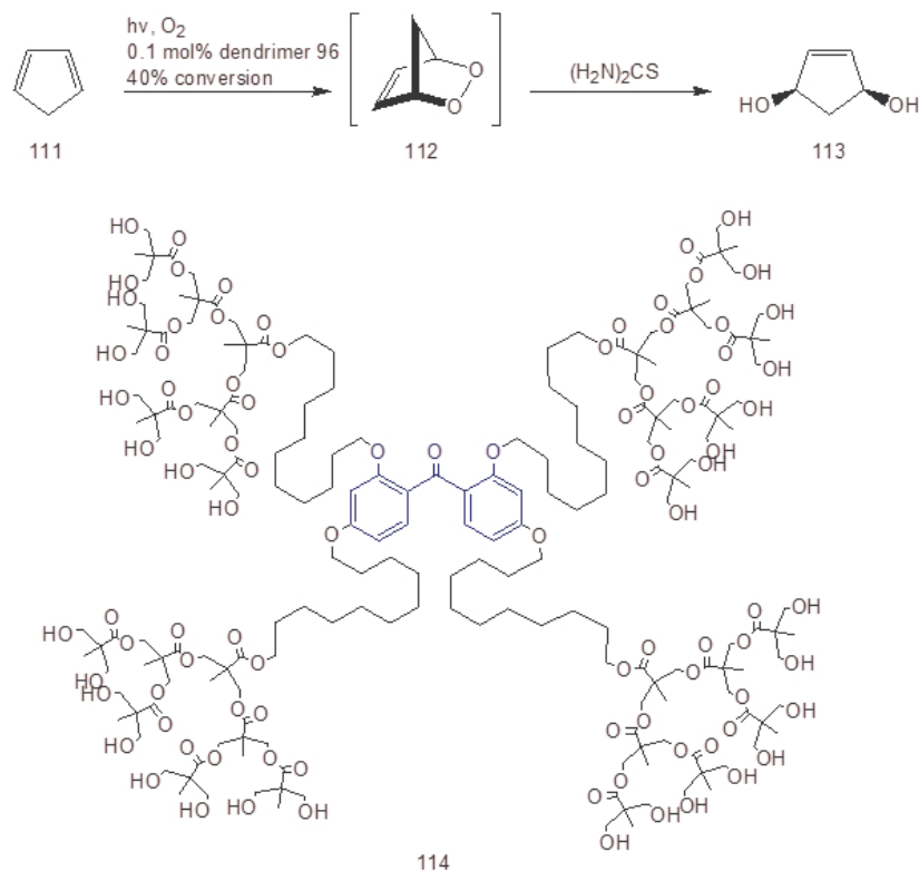
Figure 26. Singlet oxygen is generated in the benzophenone core of dendrimer 114 and reacts subsequently with 111 in a [4 + 2] cycloaddition reaction to form 112, which is reduced in situ to form diol 113 [28].
