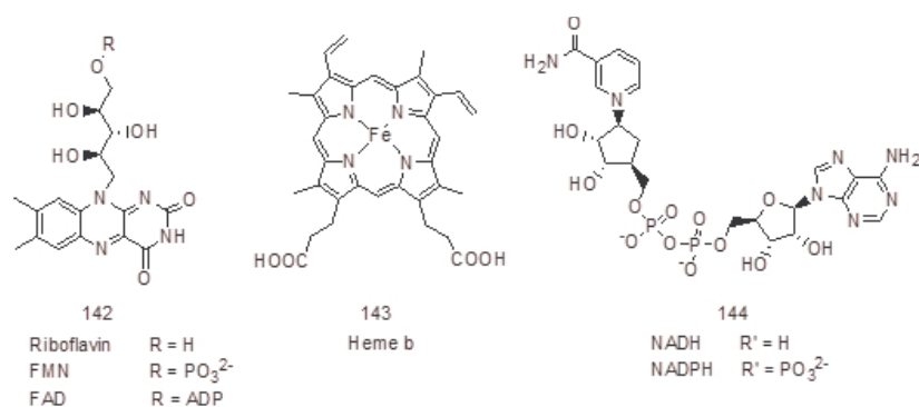
Figure 32. Examples of cofactors utilized by oxidoreductases [36].
