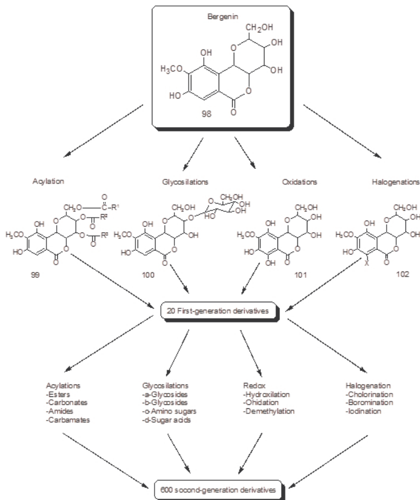
Figure 24. Iterative synthesis of a 600-member library from the flavonoid bergenin [97].
