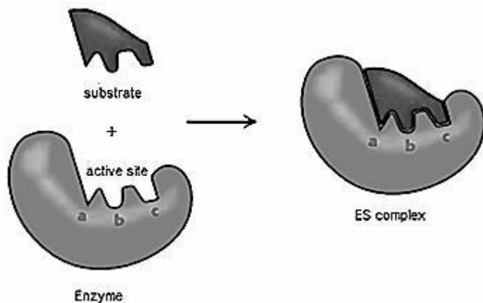
Figure 3. Lock-and-key model of enzyme-substrate binding [30].
