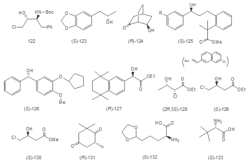
Figure 29. Some chiral building blocks obtained through bioreductions catalyzed by whole cells [8].
