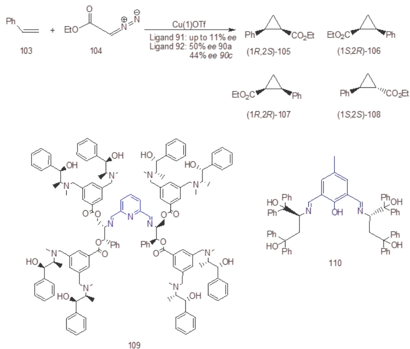
Figure 25. Brunner's dendrizyme ligands reported in 1994, active for the cyclopropanation of styrene [28].
