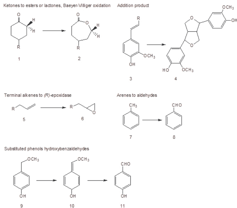
Figure 7. Examples of oxidative biotransformation reactions-monooxygenases [17].
