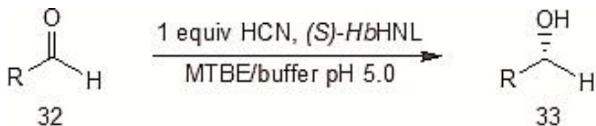
Figure 11. General enzymatic synthesis of ( S )-cyanohydrins [5].
