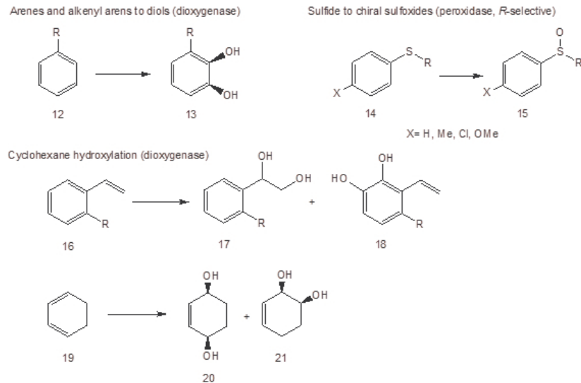
Figure 8. Examples of oxidative biotransformation reactions-dioxygenases and peroxidases [17].
