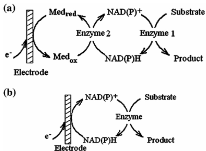
Figure 34. Cofactor regeneration with electrochemical reactions: (a) electro-enzymatic cofactor regeneration; (b) electrochemical cofactor regeneration [118].
